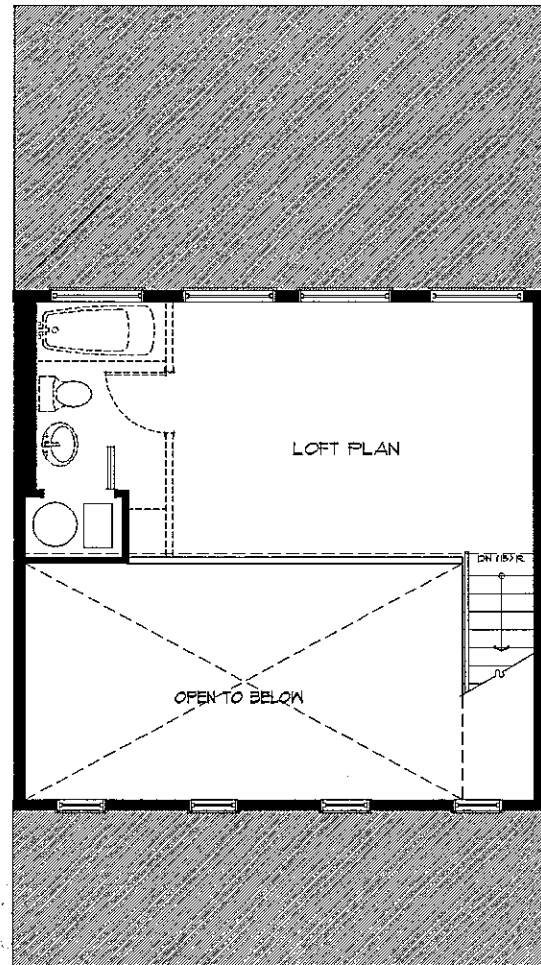
LOFT LEVEL
